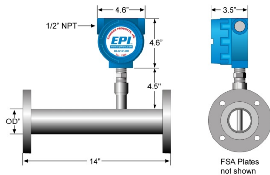
Flow Transmitter Assembly
