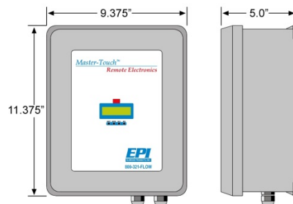
Remote Electronics Enclosure
